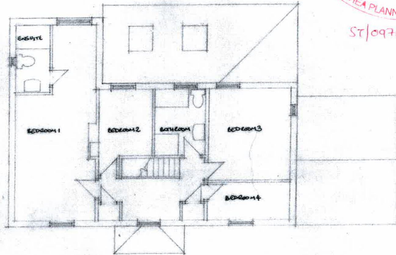
EXISTING FIRST FLOOR 1:100
